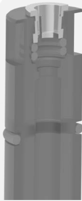
5/16" PushFit
